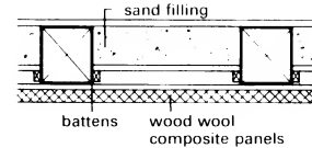
(insulation of wooden beam floor on cellar side)
